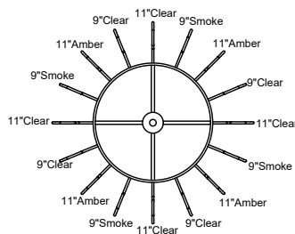
Tier#3 assemble diagram
