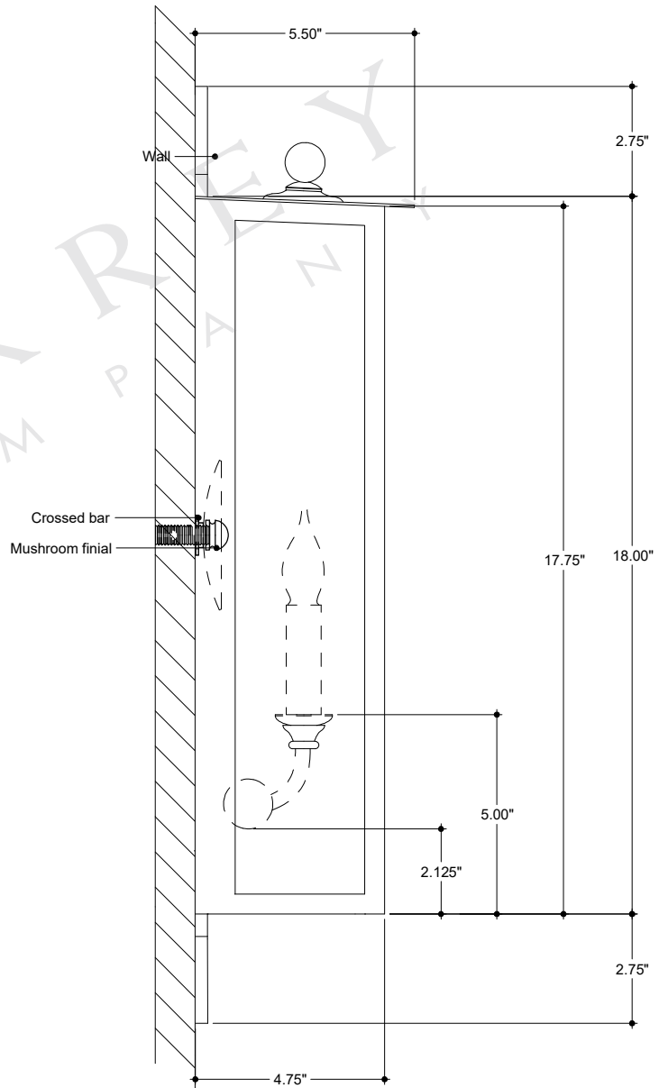
SIDE VIEW
