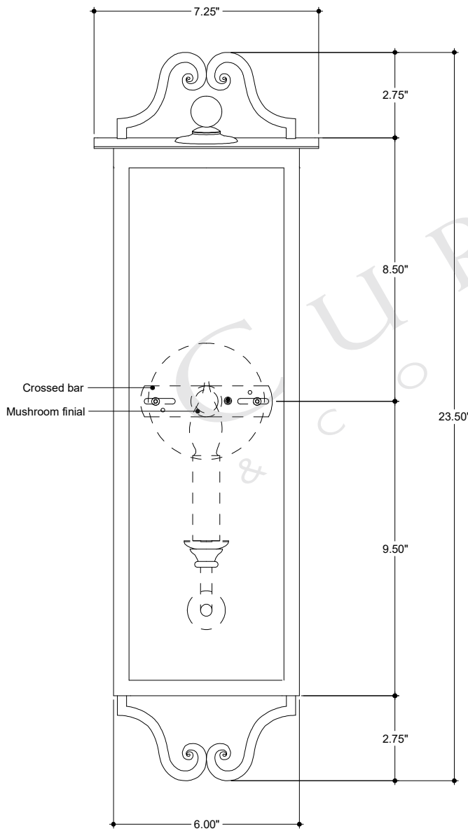
FRONT VIEW
