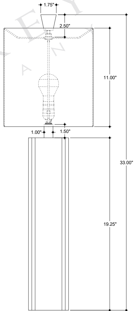
SIDE VIEW
