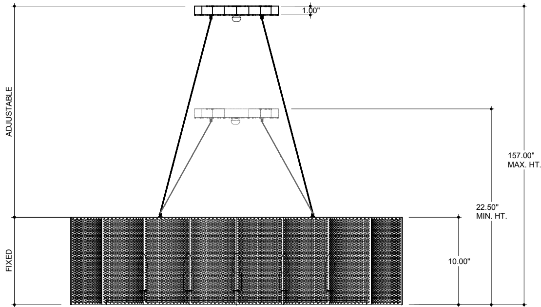
FRONT VIEW
