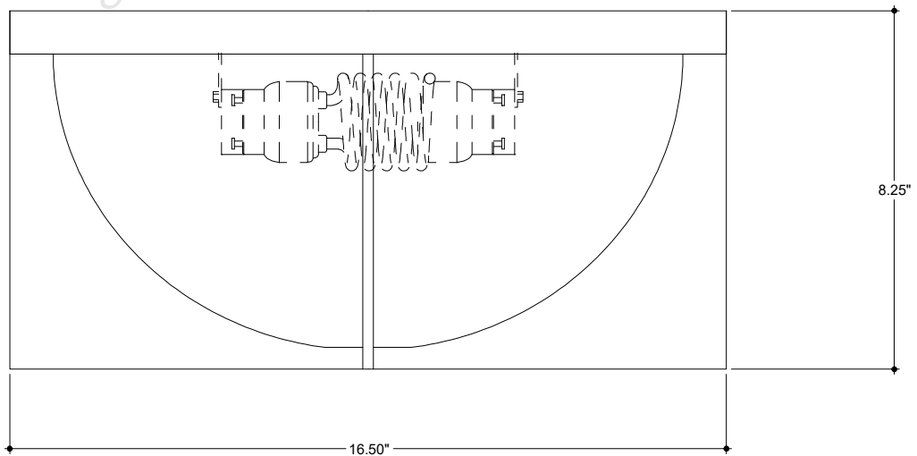
FRONT VIEW
