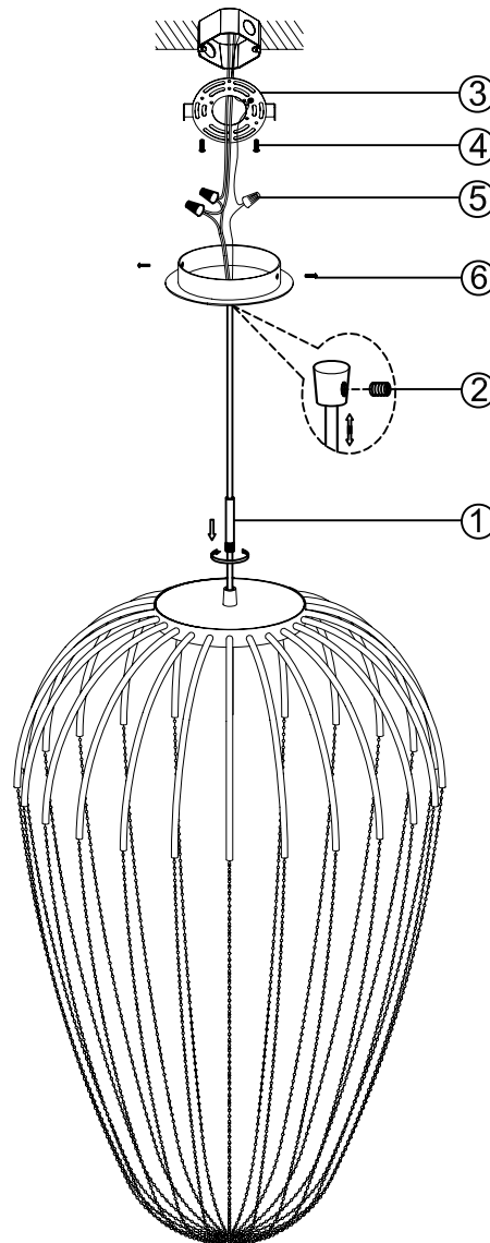
Wire connection
