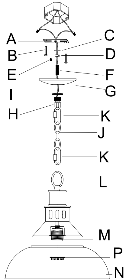
How to Identify the Fixture's Wires
