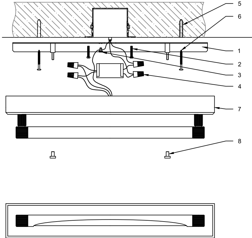
FINISHED FRONT VIEW
