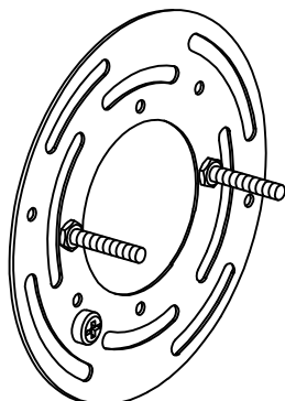
MOUNTING BRACKET
