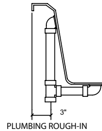
Units available Right or Left Hand Drain (Left Hand Shown)
