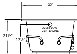
Units available Right or Left Hand Drain (Left Hand Shown)
