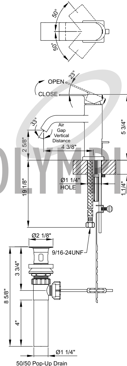
50/50 Pop-Up Drain
